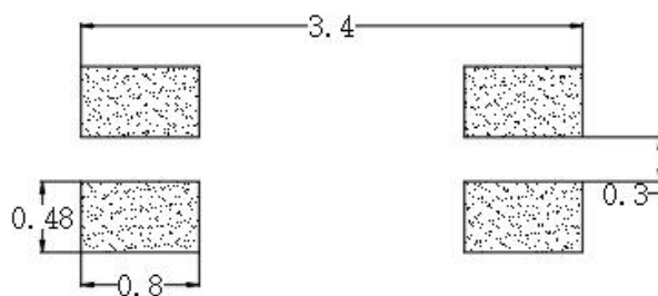
建议焊盘尺寸 Recommended Soldering Pattern
