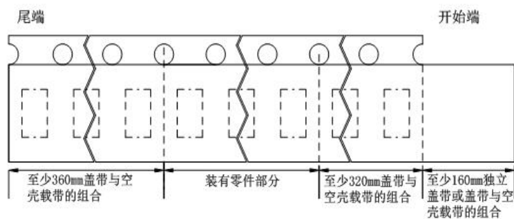
◆ 圆盘及载带卷出方向及空穴规格 Disk and carrier belt direction of roll and hole dimensions
