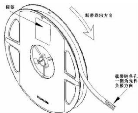
◆ 圆盘及载带卷出方向及空穴规格 Disk and carrier belt direction of roll and hole dimensions
