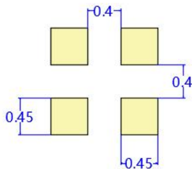
建议焊盘尺寸 Recommended Soldering Pattern
