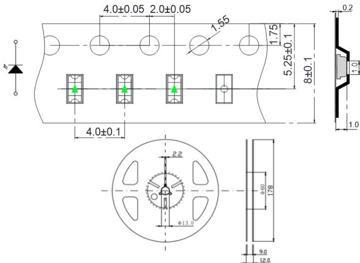
载带与圆盘尺寸 Belt and disk dimensions
