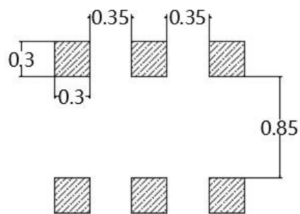
建议焊盘尺寸 Recommended Soldering Pattern
