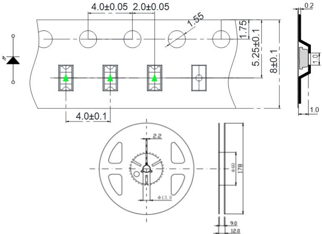
载带与圆盘尺寸 Belt and disk dimensions
