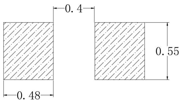
建议焊盘尺寸 Recommended Soldering Pattern
