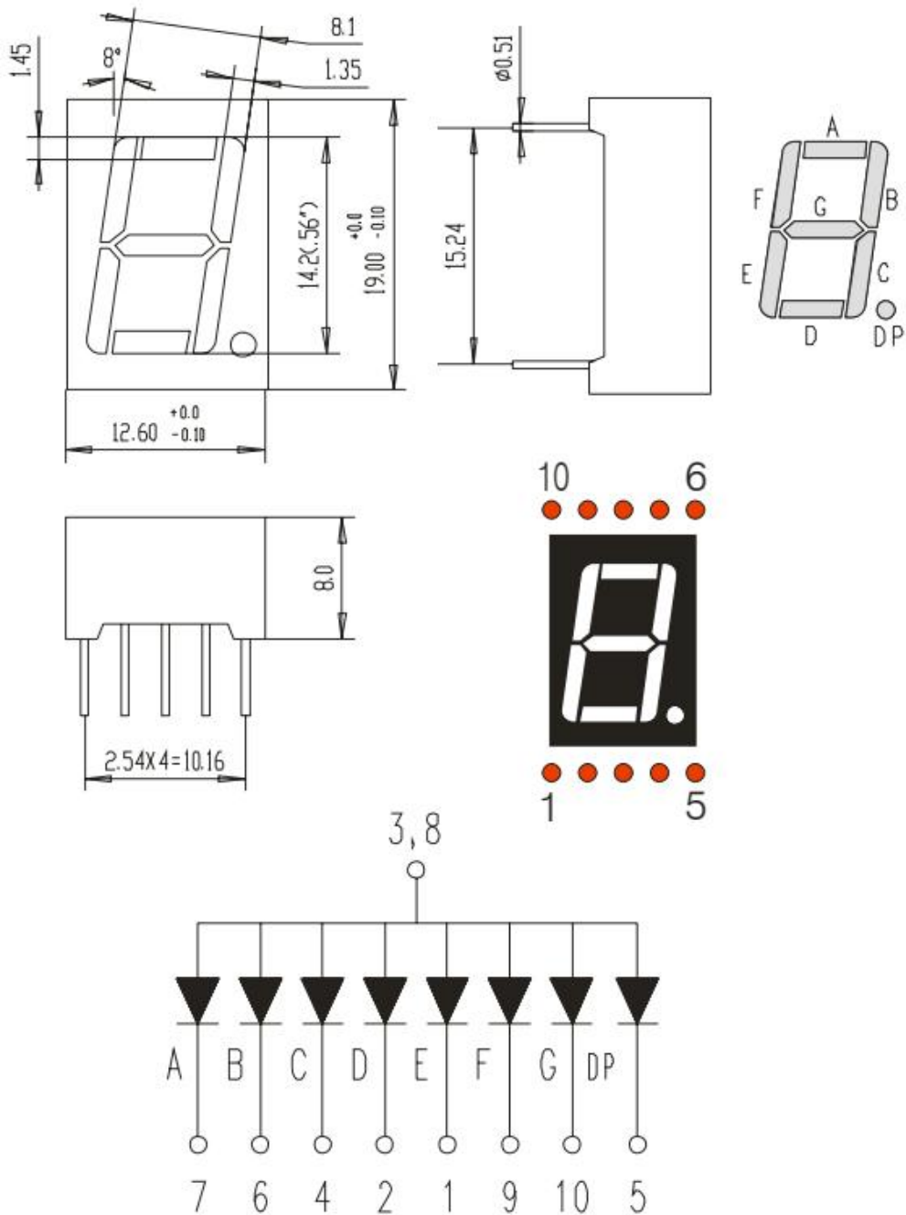
Figure Size & Circuit Principle Diagram : 12.6mm×19mm×8.0mm
