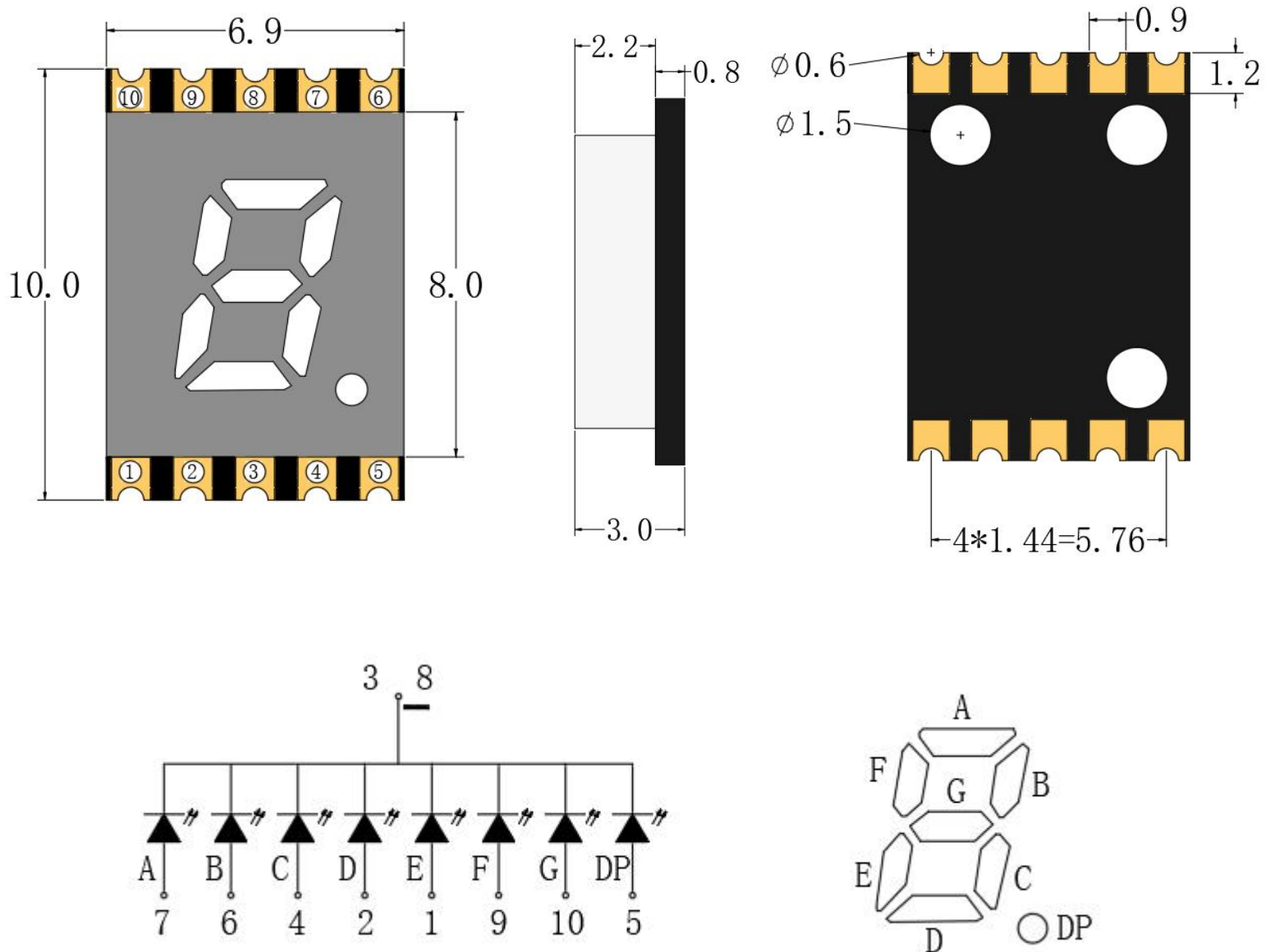
Figure Size & Circuit Principle Diagram : 10mm×6.9mm×3.0mm
