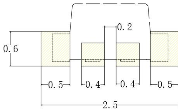
建议焊盘尺寸 Recommended Soldering Pattern
