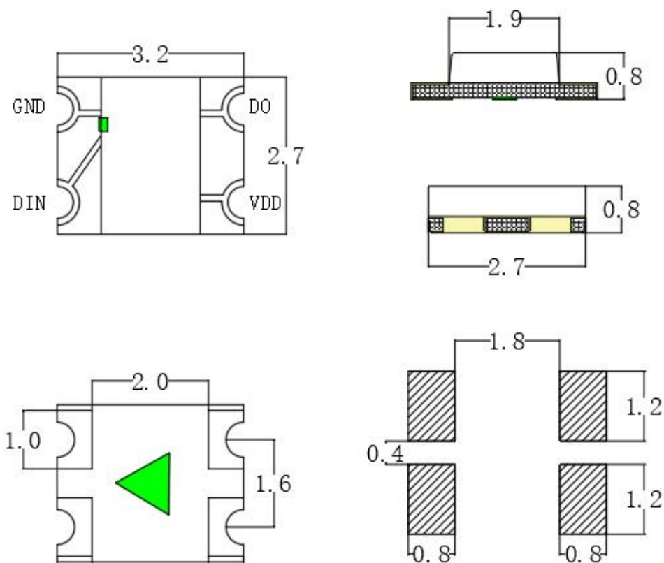
建议焊盘尺寸 Recommended Soldering Pattern
