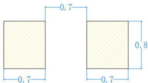
建议焊盘尺寸 Recommended Soldering Pattern
