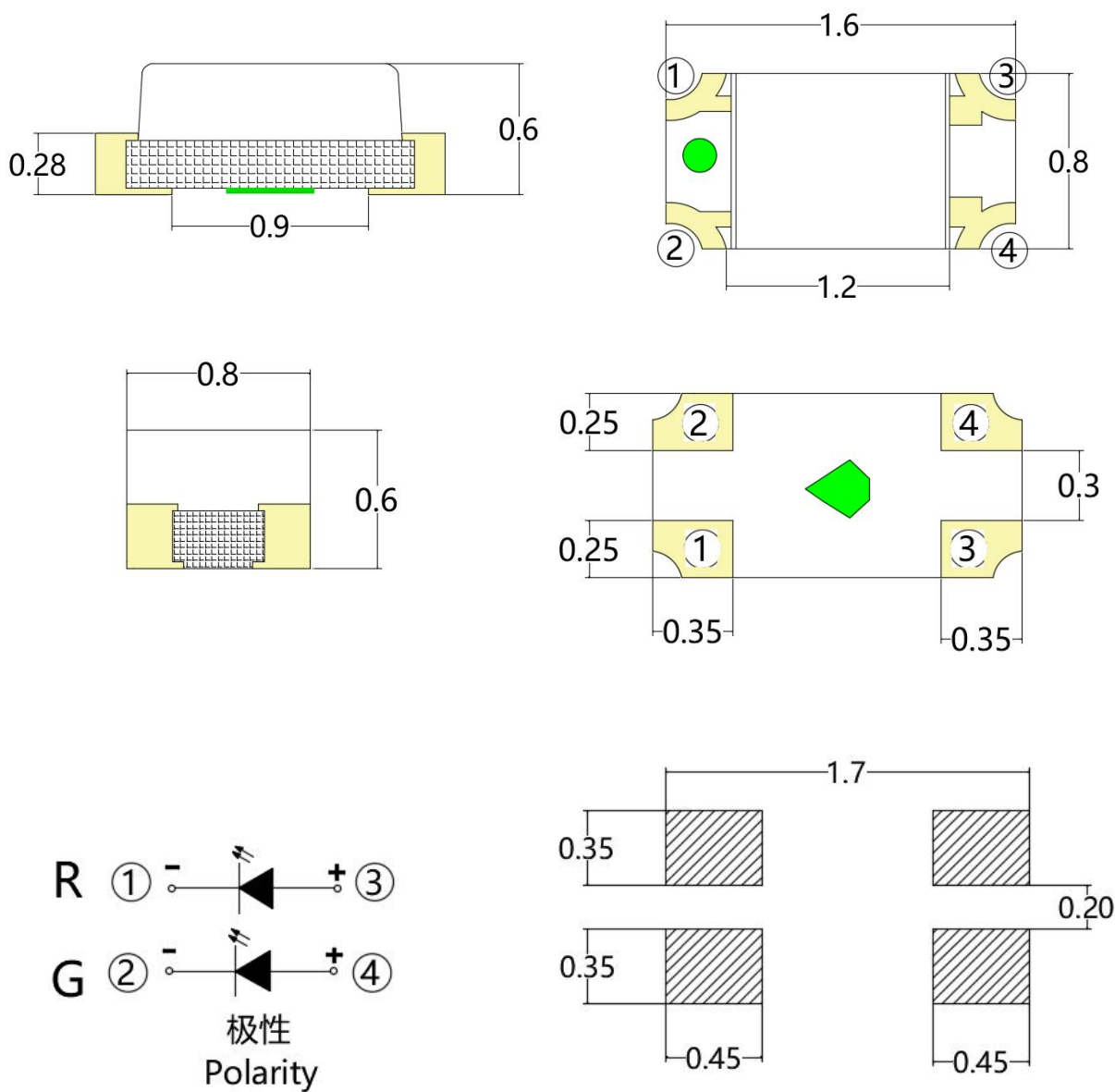
建议焊盘尺寸 Recommended Soldering Pattern
