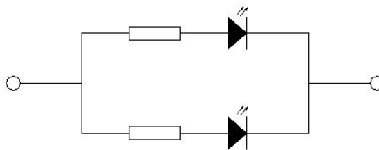
Circuit model B
