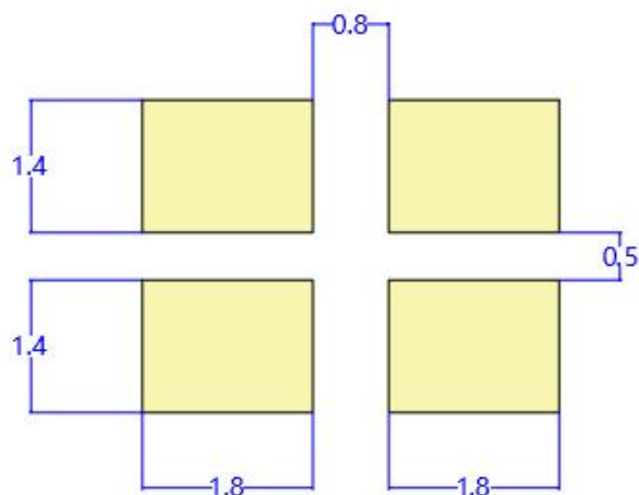
建议焊盘尺寸 Recommended Soldering Pattern
