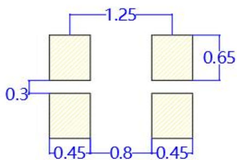
建议焊盘尺寸 Recommended Soldering Pattern
