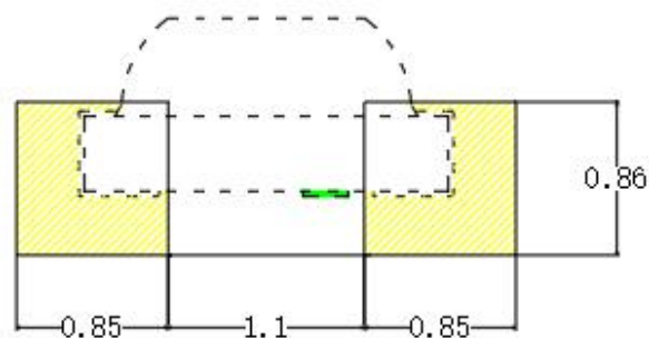
建议焊盘尺寸 Recommended Soldering Pattern
