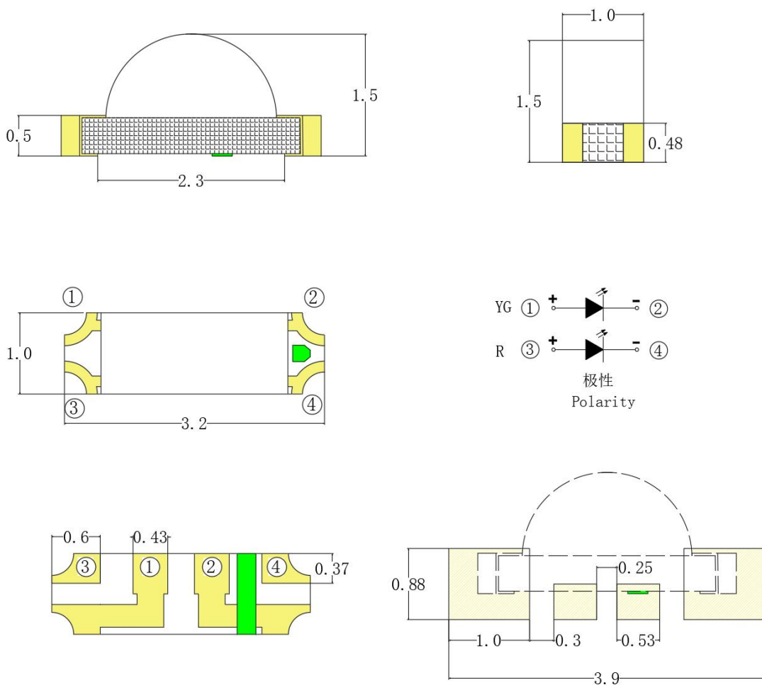
建议焊盘尺寸 Recommended Soldering Pattern
