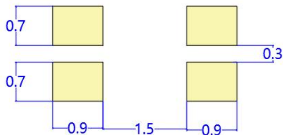
建议焊盘尺寸 Recommended Soldering Pattern
