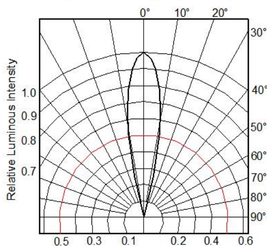
Fig.6 Radiation diagram( T_a=25^{\circ}\text{C} )
