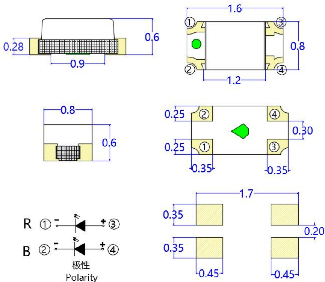
建议焊盘尺寸 Recommended Soldering Pattern
