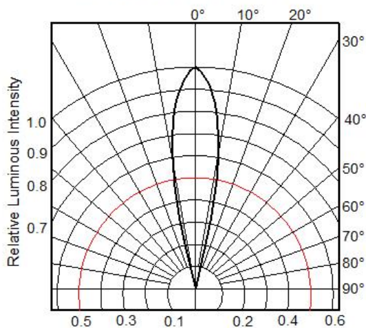
Fig.6 Radiation diagram(Ta=25°C)
