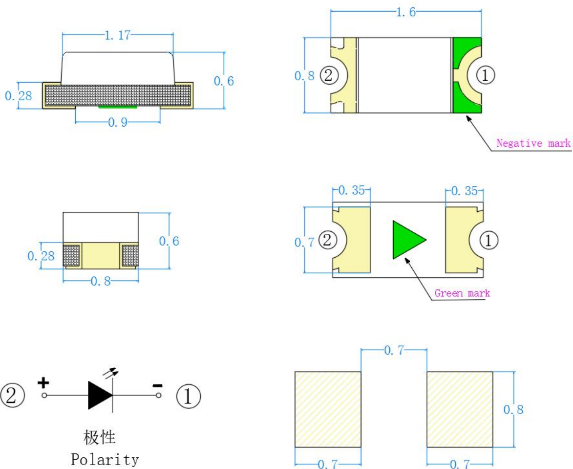
建议焊盘尺寸 Recommended Soldering Pattern
