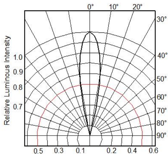
Fig.6 Radiation diagram(Ta=25°C)
